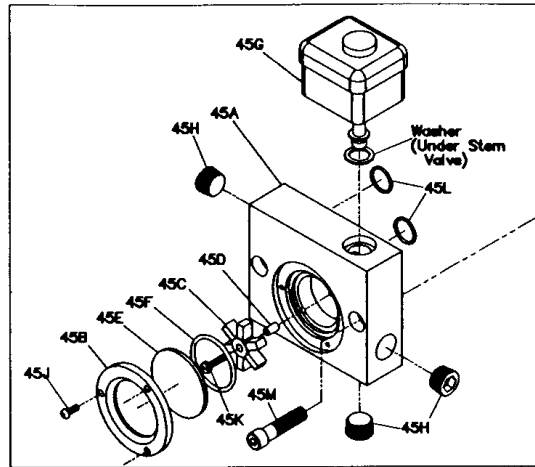
Enlarged View of Oil Manifold Assembly (45)
