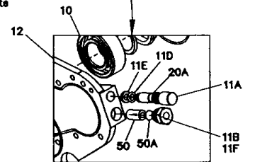
Enlarged View of Gas Ballast Valve
