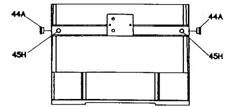
View 'A' - Rear View of Pump Housing (Oil Manifold Assembly Not Shown)
