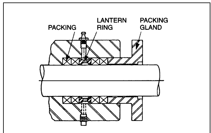
Figure 4-1. Cross Section of Packing Retainer
